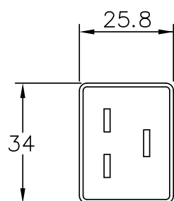
IEC C20
